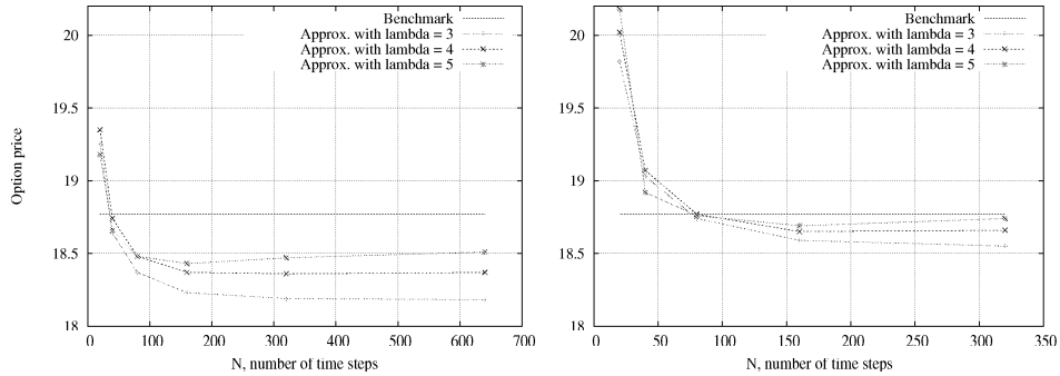
Fig. 2 Approximate prices of a Swing option with 2 exercise rights and \delta = \frac{2}{10} , with p = 5 (left) and p = 10 (right)
