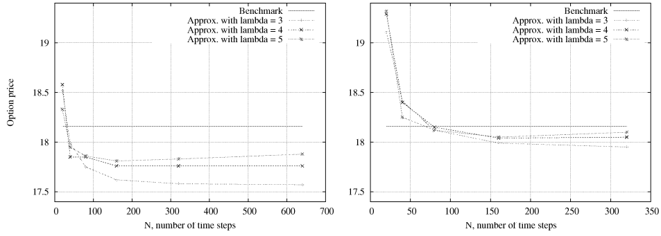
Fig. 3 Approximate prices of a Swing option with 2 exercise rights and \delta = \frac{3}{10} , with p = 5 (left) and p = 10 (right)
