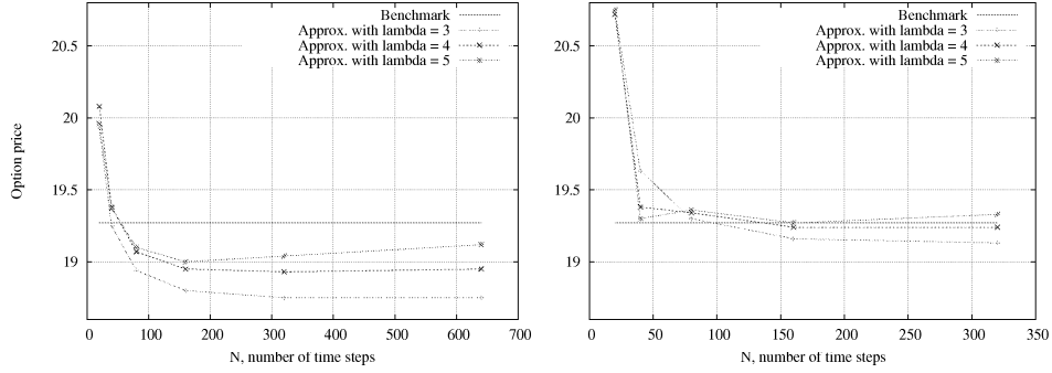
Fig. 1 Approximate prices of a Swing option with 2 exercise rights and \delta = \frac{1}{10} , with p = 5 (left) and p = 10 (right)
