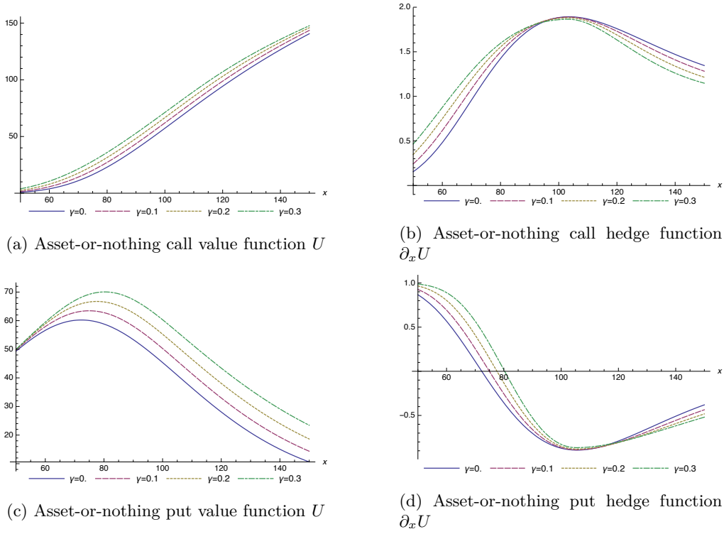
Figure 5: Digital options: numerical approximation of f^* -PDE solution U at final time for different \gamma .
