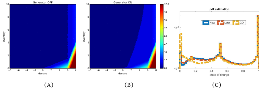
FIGURE 4. In the figure above we show, in the two left-most panels, an example of control map produced by the Regress Later algorithm at time t = 0 . Notice the difference depending on the state of the generator. In the right-most panel we display the estimated probability density function of the state of charge of the battery associated with the use of the three policies. It can be observed that Regress Later and Grid discretization induce very similar distributions.
