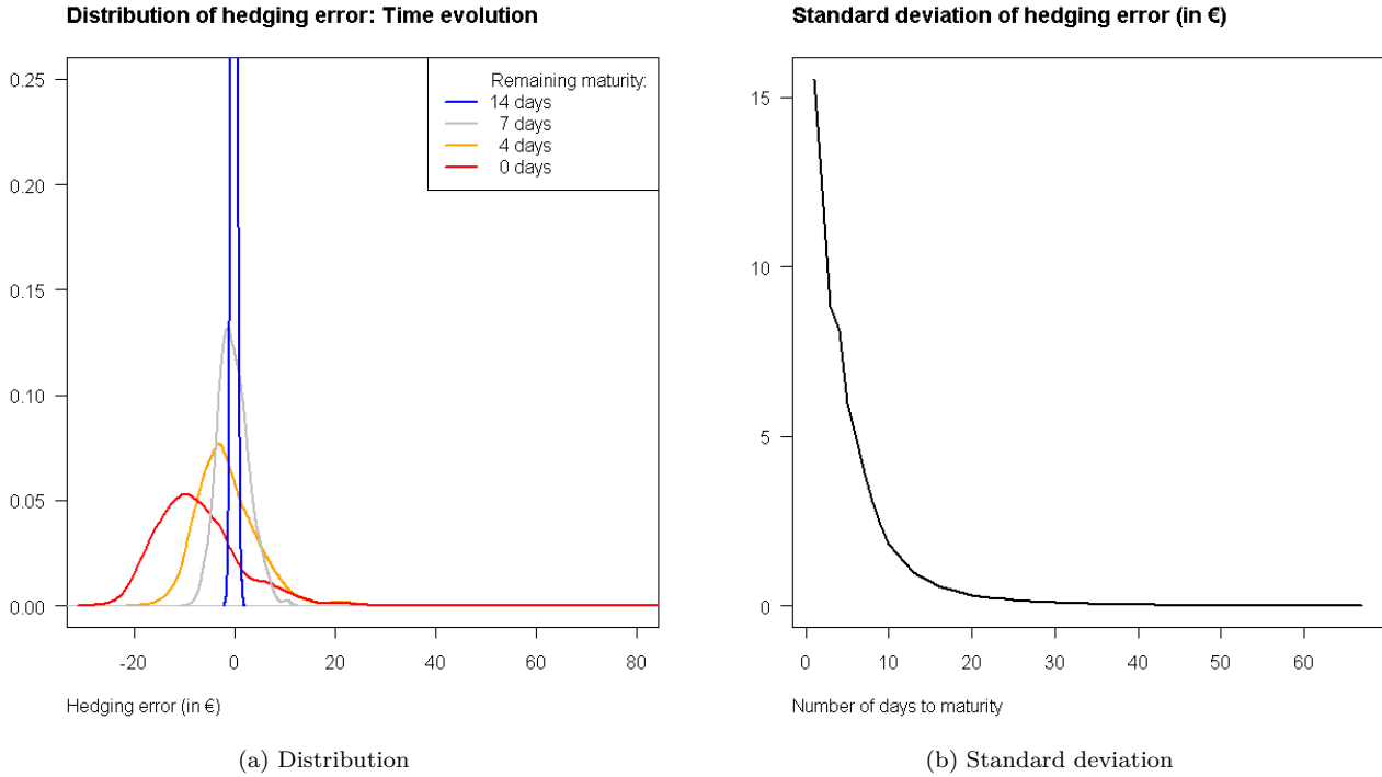
Figure 4.4: Hedging error
