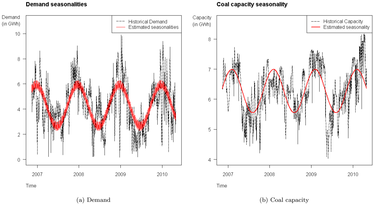
Figure 4.1: Seasonalities estimates
