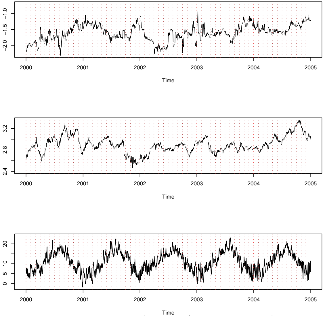
Fig. 1. Daily series of gas log-prices g_t (upper panel), Brent log-prices b_t (middle panel) and temperatures T_t (lower panel).
