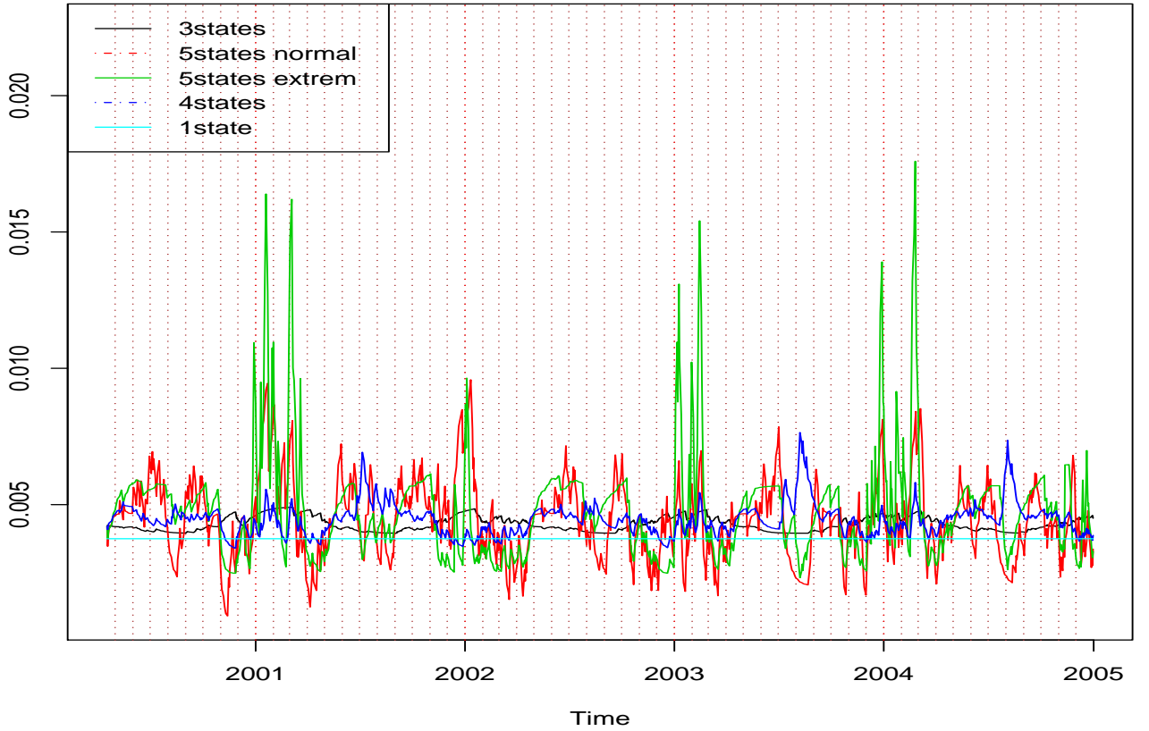
Fig. 5. Unconditional variance E\epsilon_t^2 for the estimated models.
