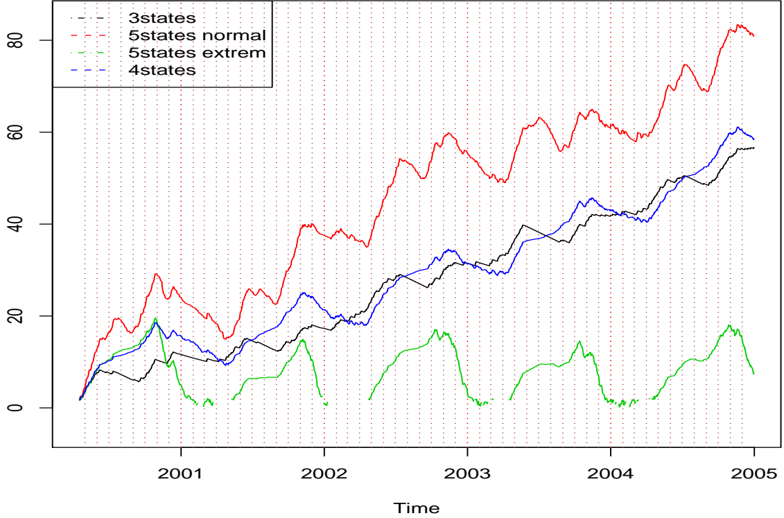
Fig. 6. Unconditional kurtosis in logarithms, \log\{E\epsilon_t^4/E(\epsilon_t^2)^2\} . Missing values in the curve of Model (16) are due to kurtosis approaching zero.
