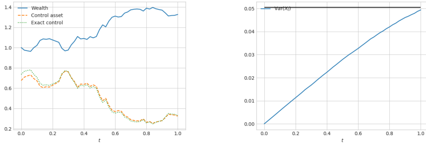
FIGURE 5. Sample trajectory of the controlled process X_t^\alpha and the control for problem (28) (left). Variance \text{Var}(X_t) estimated with 50000 samples for problem (28) (right) with \Lambda = 10
